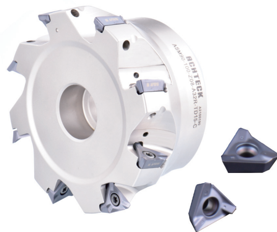
Application: Pocket milling Solution: ASM90-TD15
