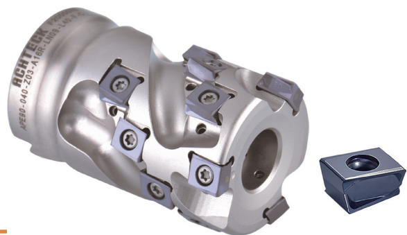
Application: Profile/main hole rough milling Solution: Achteck porcupine milling cutter APE90-LN09/13/AO12
