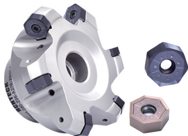
Application: Rough face milling Solution: Achteck XNMU 07 /09 series
