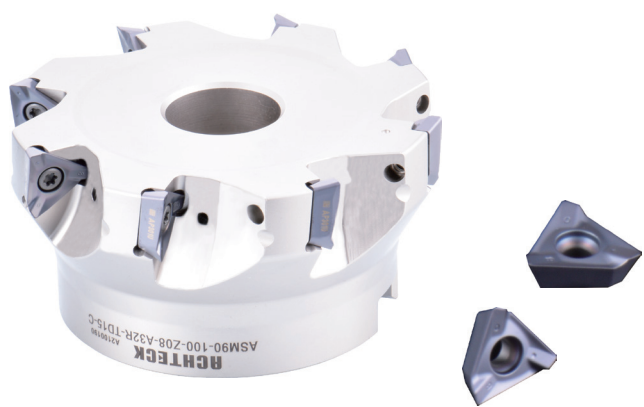
Application: Pocket rough milling Solution: Achteck TDMT 1505 series
